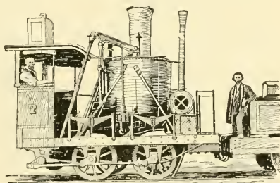
*THE DAVIS "GRASSHOPPER" TYPE OF LOCOMOTIVE ON B. & O. R. R., 1832
